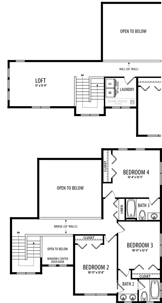
Upper Level
