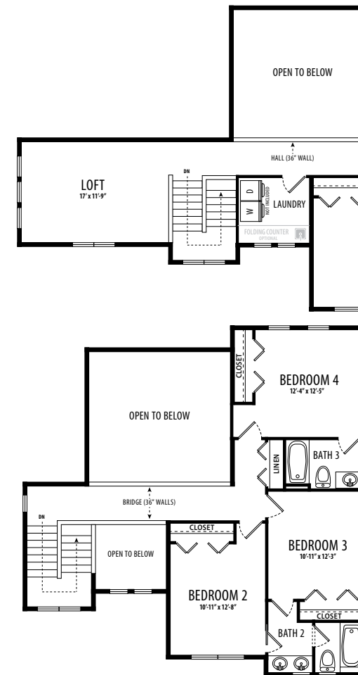
Upper Level
